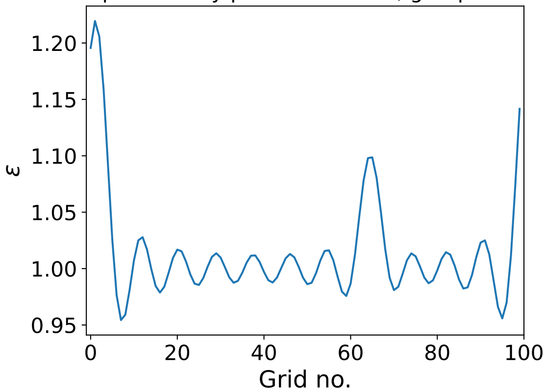
GRCWA permittivity profile. n_G = 25 , grid points = 100
